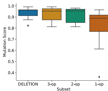
Fig. 5. Mutation coverage: Proportion of FULL mutants detected by the subset-adequate test suite.
